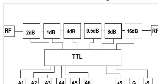
Functional Diagram
